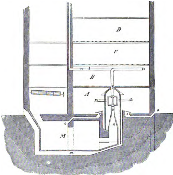
Fig. 364.—Seed-kiln with fixed trays.
